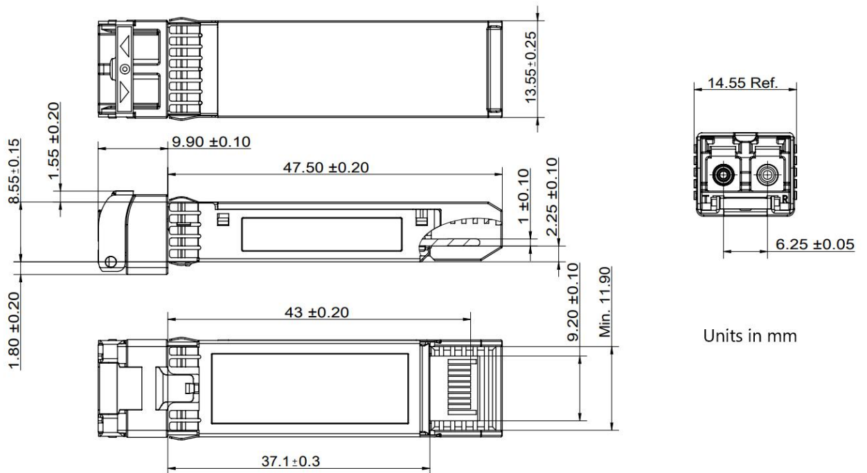
Figure2. Mechanical Outline
